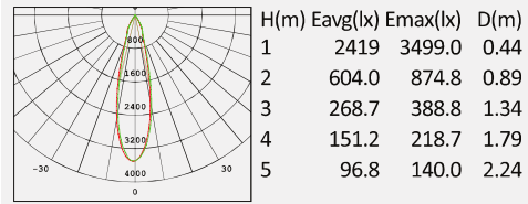
No: 4019S/4020S-10W LED CREE COB LED 1*10W 888lm Clear Glass 24° Class I, IP65
