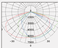
No: 7015-150W LED Lumileds LED 150W 22383lm Clear Glass 148° Class I, IP65
