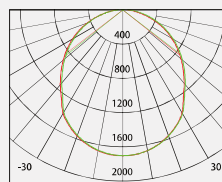
No: 1000C-60W LED Lumileds LED 60W 4015lm Opal PC 104.19° Class I, IP65
