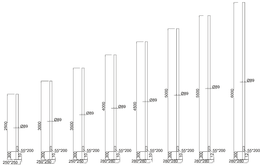
Hot-galvanised steel Cylindrical poles
