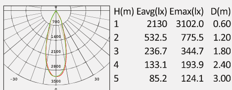
No: 4019S/4020S-15W LED CREE COB LED 1*15W 1165lm Clear Glass 36° Class I, IP65
