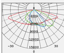
No: 7022-150W LED Lumileds LED 150W 20273lm Clear Glass 158° Class I, IP65
