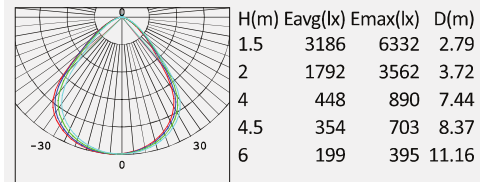
No: 8102-200W LED SMD 2835 200W 28467lm Clear PC 90° Class I, IP66
