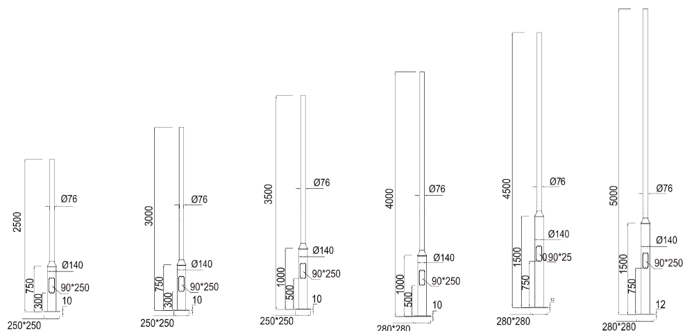
Hot-galvanised steel Tapered Poles
