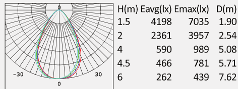
No: 8102-150W LED SMD 2835 150W 21322lm Clear PC 60° Class I, IP66
