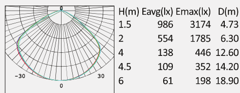
No: 8102-150W LED SMD 2835 150W 21489lm Clear PC 120° Class I, IP66
