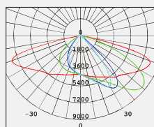
No: 7021-120W LED Lumileds LED 120W 15955lm Clear Glass 155° Class I, IP65
