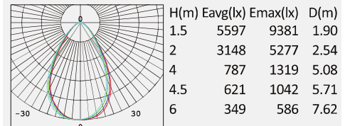
No: 8102-200W LED SMD 2835 200W 28429lm Clear PC 60° Class I, IP66
