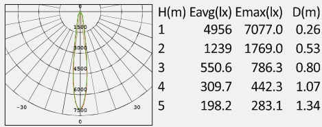
No: 4019S/4020S-10W LED CREE COB LED 1*10W 917lm Clear Glass 15° Class I, IP65
