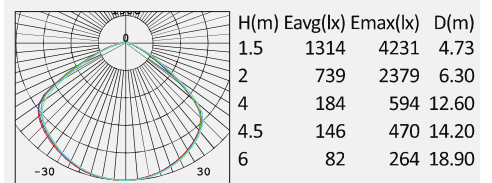
No: 8102-200W LED SMD 2835 200W 28645lm Clear PC 120° Class I, IP66
