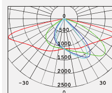
No: 7018-40W LED Lumileds LED 40W 4045lm Clear Glass 156^{\circ} Class I, IP65
