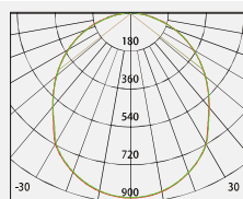
No: 1000C-30W LED MTC LED 30W 2308lm Opal PC 104.19° Class I, IP65
