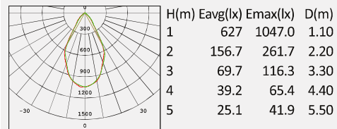
No: 4019S/4020S-10W LED CREE COB LED 1*10W 917lm Clear Glass 60° Class I, IP65
