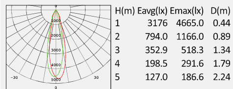
No: 4019S/4020S-15W LED CREE COB LED 1*15W 1197lm Clear Glass 24° Class I, IP65
