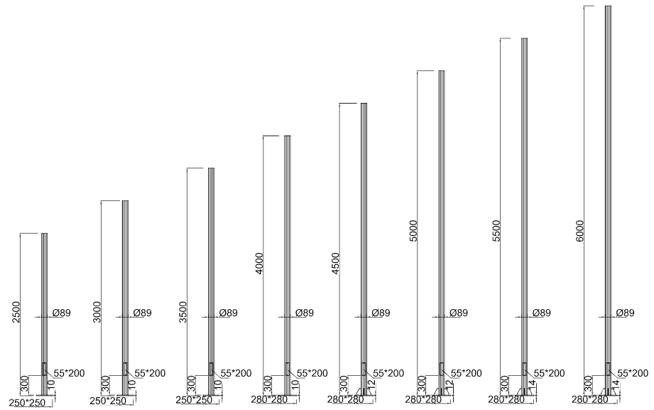
Extruded Aluminum(with ribs) Cylindrical poles
