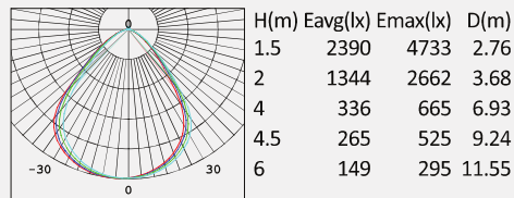
No: 8102-150W LED SMD 2835 150W 21120lm Clear PC 90° Class I, IP66
