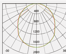
No: 1000D-60W LED Lumileds LED 60W 4015lm Opal PC 104.19° Class I, IP65
