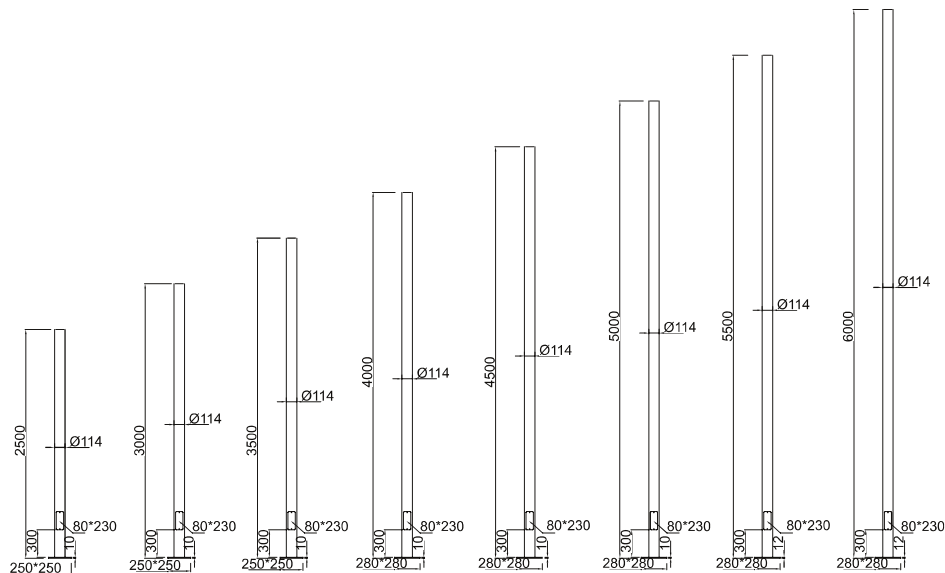
Hot-galvanised steel Cylindrical poles
