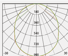
No: 1000D-30W LED MTC LED 30W 2308lm Opal PC 104.19° Class I, IP65
