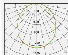
No: 1000C-45W LED Lumileds LED 45W 3325lm Opal PC 104.19° Class I, IP65
