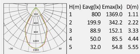
No: 4019S/4020S-15W LED CREE COB LED 1*15W 1191lm Clear Glass 60° Class I, IP65
