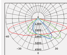
No: 7020-90W LED Lumileds LED 90W 12062lm Clear Glass 155^{\circ} Class I, IP65
