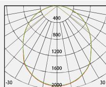
No: 1000D-80W LED Lumileds LED 80W 5044lm Opal PC 104.19° Class I, IP65
