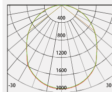
No: 1000C-80W LED Lumileds LED 80W 5044lm Opal PC 104.19° Class I, IP65
