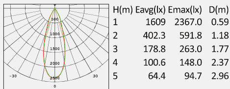
No: 4019S/4020S-10W LED CREE COB LED 1*10W 874lm Clear Glass 36° Class I, IP65
