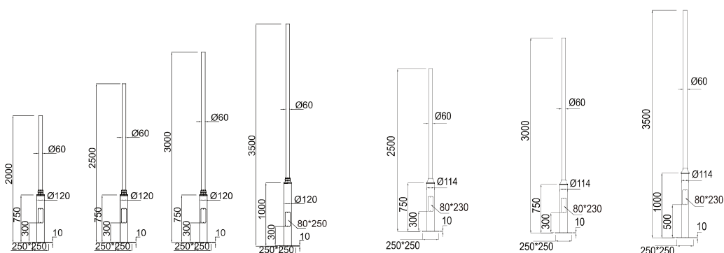
Extruded Aluminium Tapered Poles
