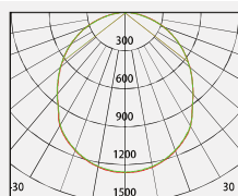
No: 1000D-45W LED Lumileds LED 45W 3325lm Opal PC 104.19° Class I, IP65
