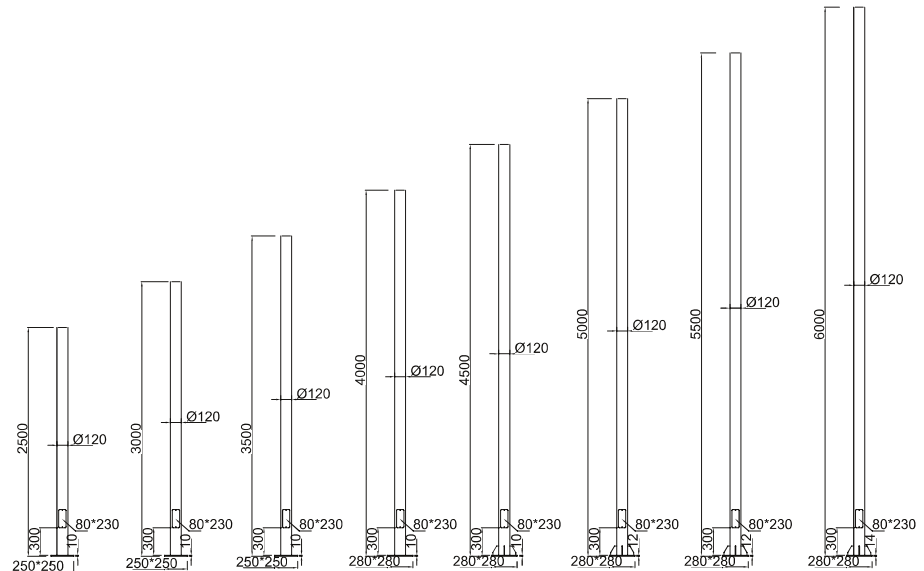
Extruded Aluminum Cylindrical poles
