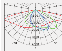
No: 7019-60W LED Lumileds LED 60W 7790lm Clear Glass 159^{\circ} Class I, IP65
