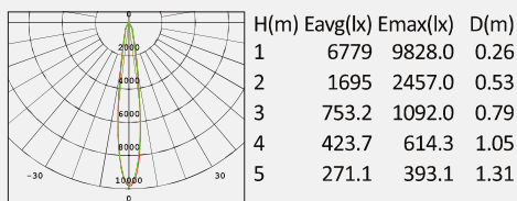
No: 4019S/4020S-15W LED CREE COB LED 1*15W 1245lm Clear Glass 15° Class I, IP65
