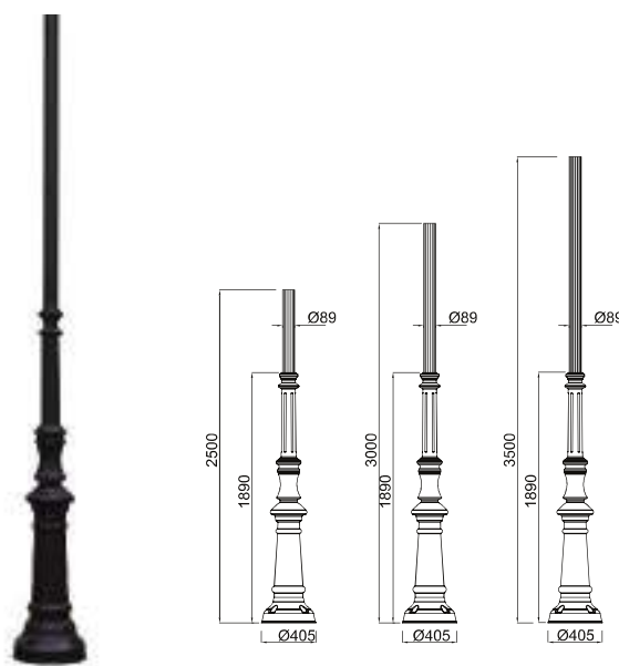
Sanding cast base and Extruded Aluminium Pole
