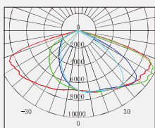
No: 7015-180W LED Lumileds LED 180W 25309lm Clear Glass 148° Class I, IP65
