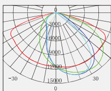
No: 7015-200W LED Lumileds LED 200W 33223lm Clear Glass 148° Class I, IP65
